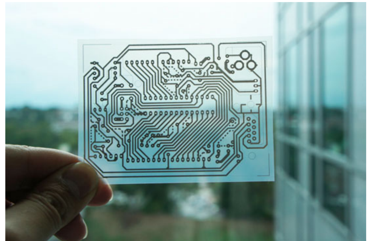
This printed circuit, developed by Georgia Tech, allows users, professionals and amateurs, to create cheaper and faster prototype electronics.
